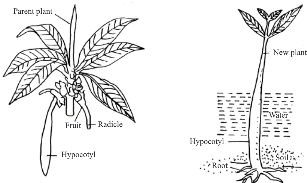
Fig 20.5 Viviparous Germination
